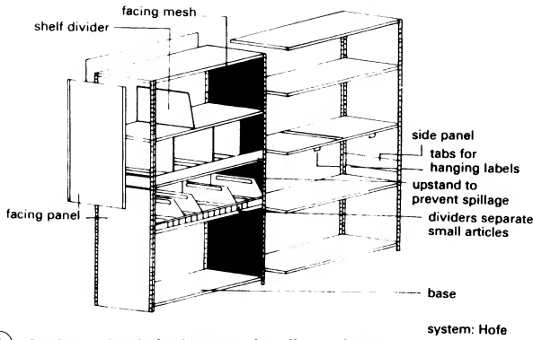
1 Angle-section bolted system for all-round use
